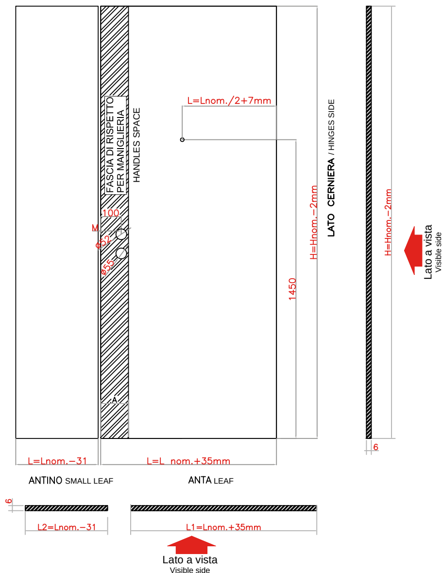
PANNELLI INTERNI / INTERNAL PANELS
